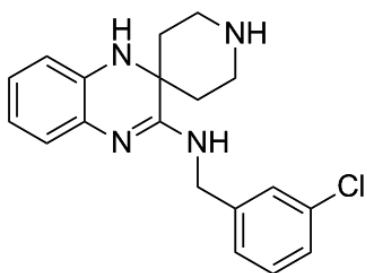
PC-4316401, DMSO-d6
